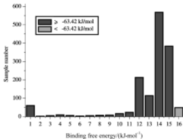
Figure 5 Histogram of virtual screening (1: >462 kJ/mol; 2: <462 and \geq 420 kJ/mol; 3: <420 and \geq 378 kJ/mol; 4: <378 and \geq 336 kJ/mol; 5: <336 and \geq 294 kJ/mol; 6: <294 and \geq 252 kJ/mol; 7: <252 and \geq 210 kJ/mol; 8: <210 and \geq 168 kJ/mol; 9: <168 and \geq 126 kJ/mol; 10: <126 and \geq 84 kJ/mol; 11: <84 and \geq 42 kJ/mol; 12: <42 and \geq 0 kJ/mol; 13: <0 and \geq -21 kJ/mol; 14: <-21 and \geq -42 kJ/mol; 15: <-42 and \geq -63.42 kJ/mol; 16: <-63.42 kJ/mol).
